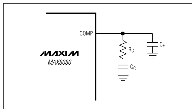
Figure 6. Compensation Components
