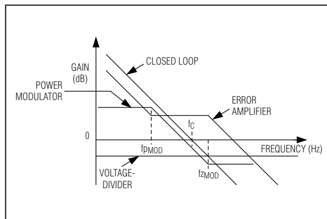
Figure 7. Simplified Gain Plot for the f_{ZMOD} > f_C Case
