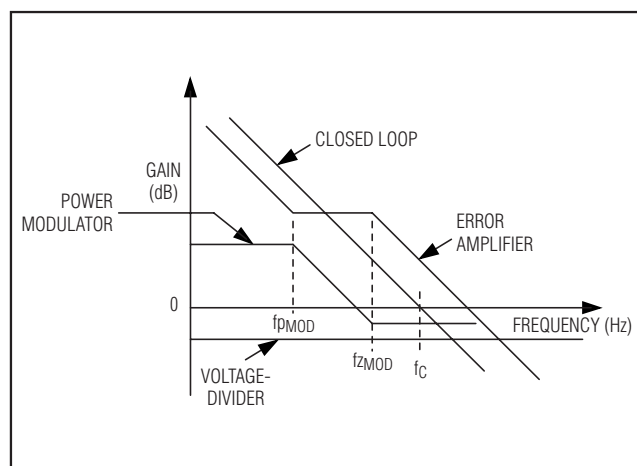
Figure 8. Simplified Gain Plot for the f_{ZMOD} < f_C Case
