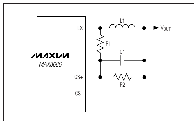
Figure 5. Current Sense Using the Inductor's DC Resistance
