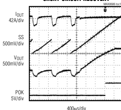
SHORT-CIRCUIT RECOVERY
